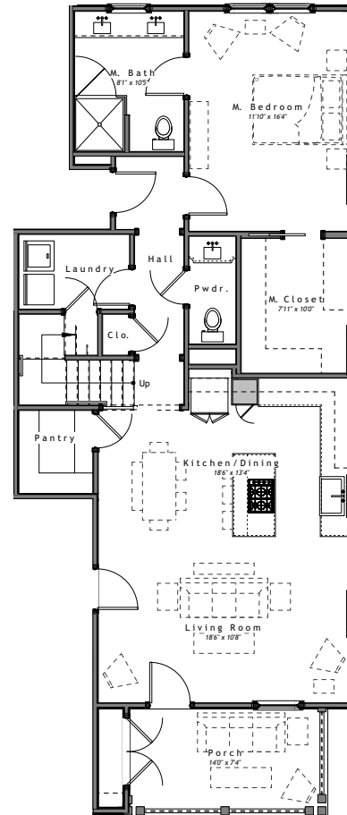
Standard Floor Plan
